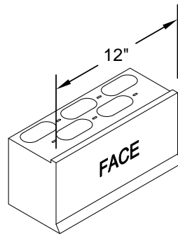
END CAP LEFT HAND SHOWN
