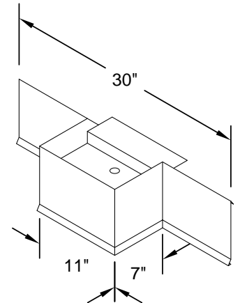
SUMP 2 PIECE ASSEMBLY
