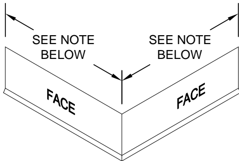
OUTSIDE MITER
