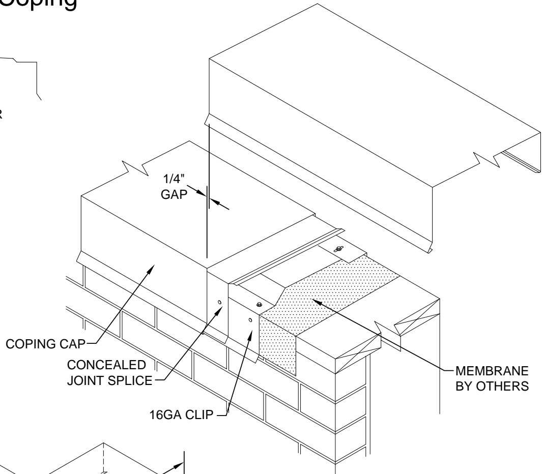
CLIP PROFILE FOR WALLS 20" TO 32"
