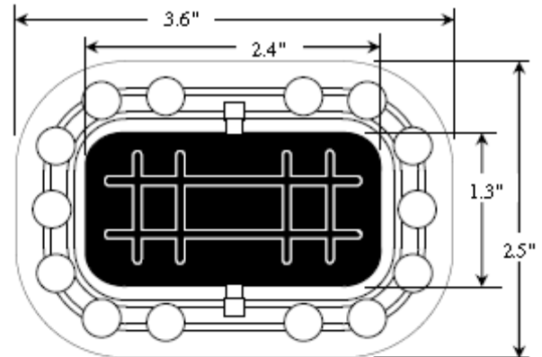
Fastener (typical)
