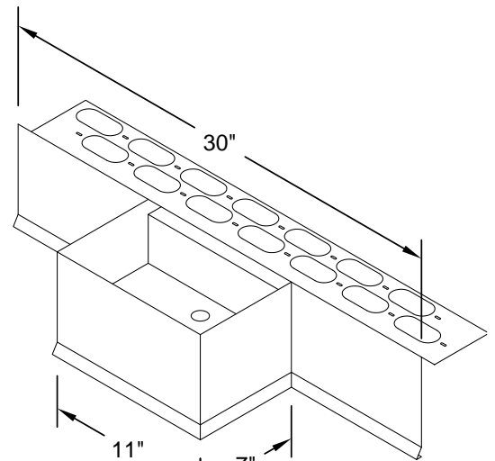
SUMP 2 PIECE ASSEMBLY
