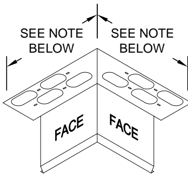
INSIDE MITER
